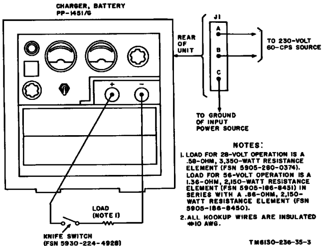
Figure 3-2. Two hundred and thirty volts, 60-cps input power test connection diagram.
