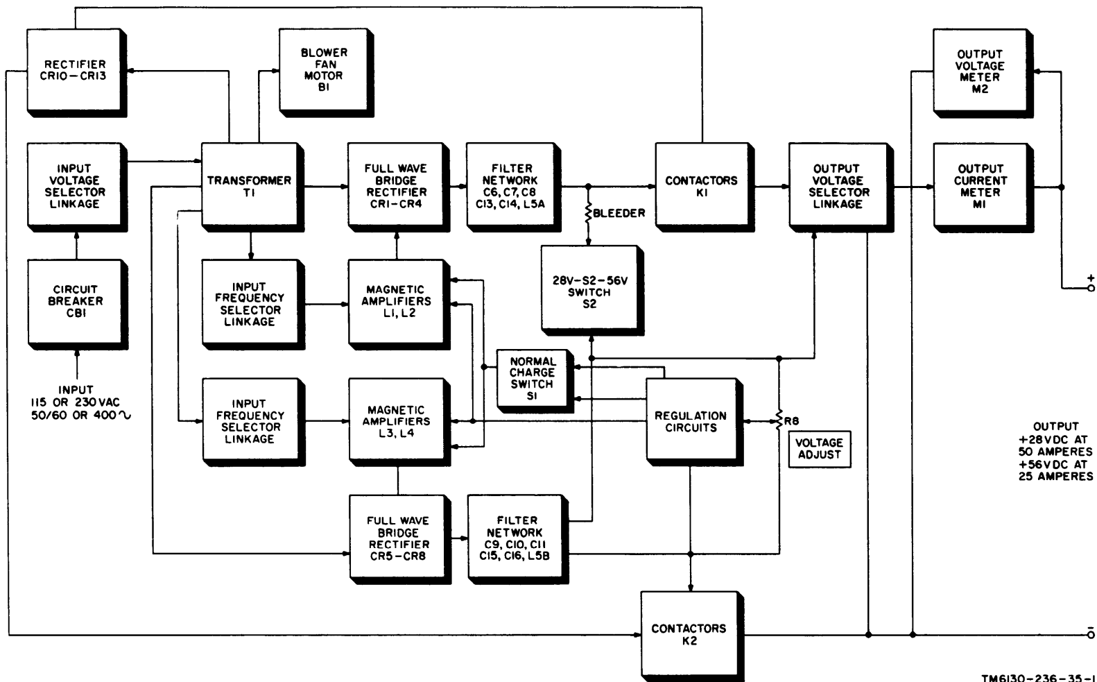
Figure 1-1. Block diagram
