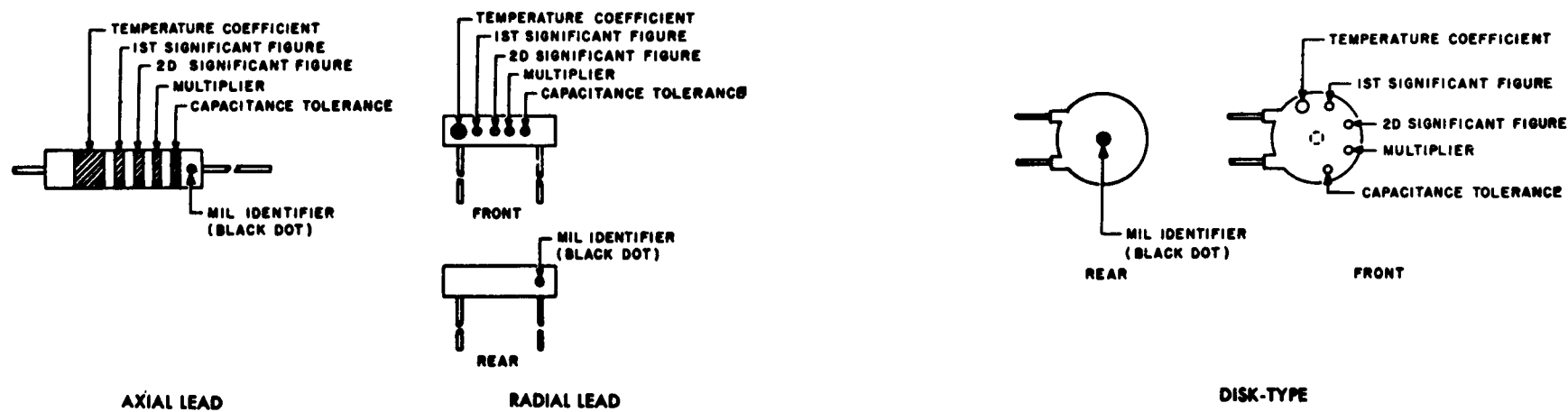
Figure 4-2. Color code marking for MIL STD capacitors.
