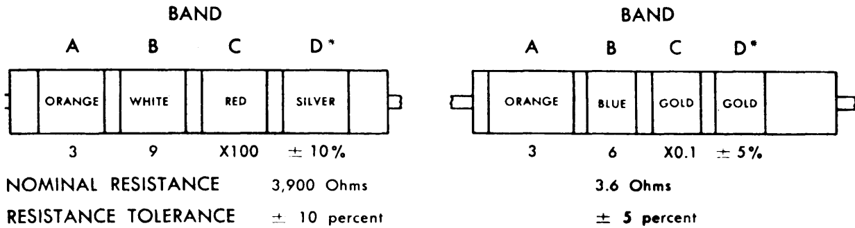
Figure 4-1. Color code marking for MIL STD resistors.
