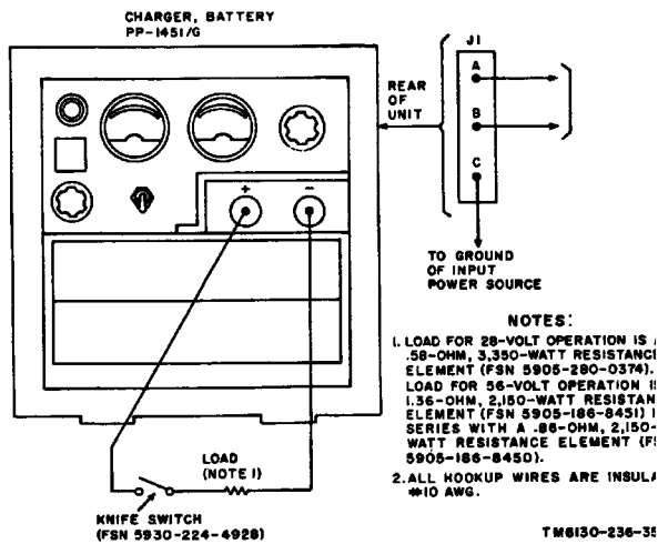
Figure 3-2. One hundred and fifteen volts, 100-ops input power test connec diagram.
