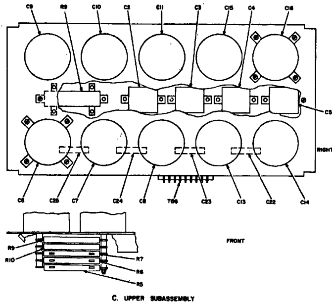
Figure 4-3. Charger, Battery PP-1451/G, parts location.
