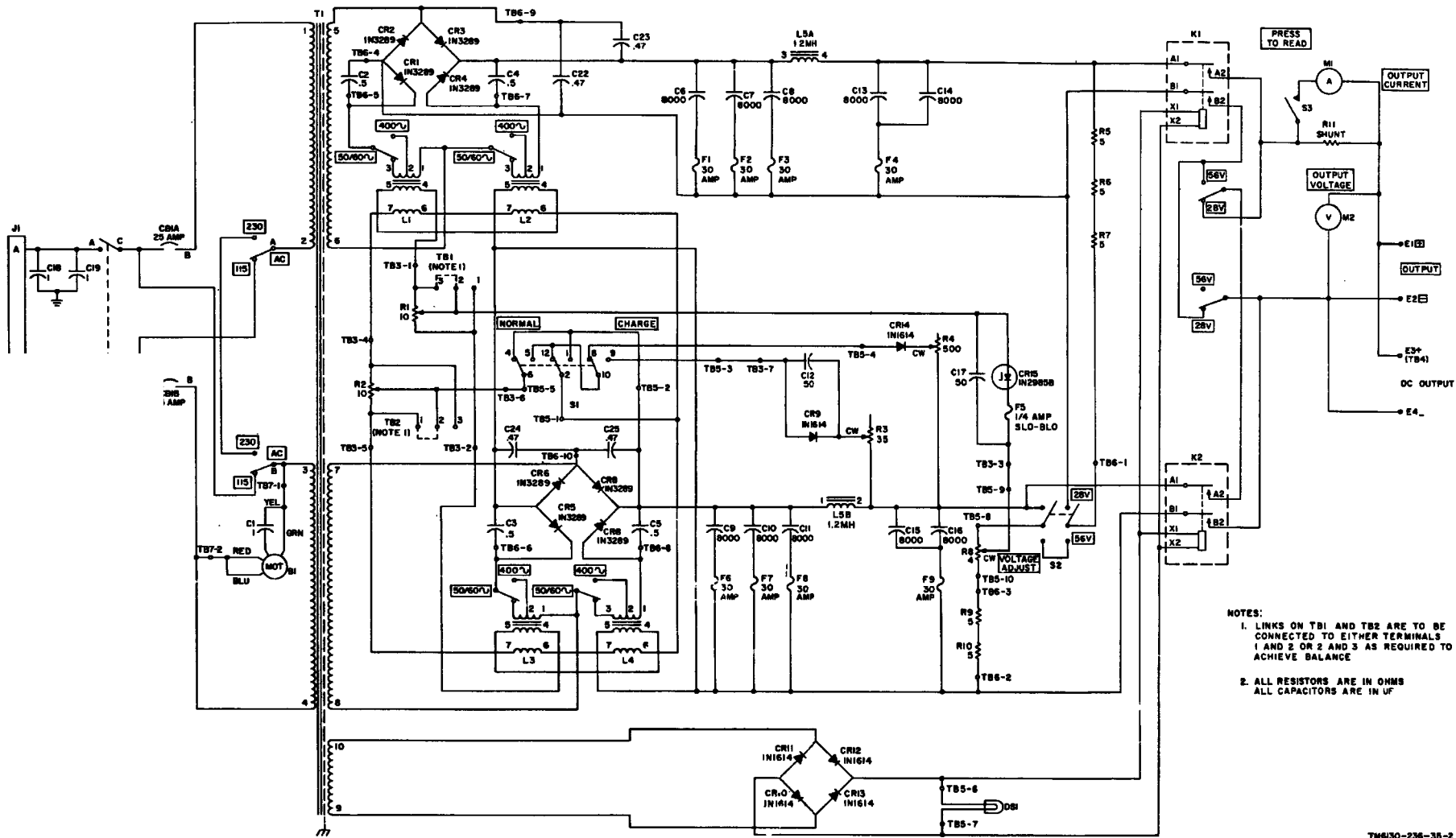
Figure 4-4. Charger, Battery PP-1151/G, schematic diagram.
